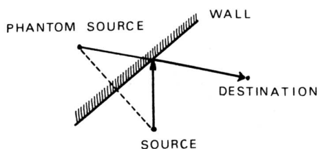
Figure 7. Diagram of a sound ray going from a sound source to a destination listener via a wall reflection. Just as in the case of light, we can think of the reflected sound as originating from a "phantom" source which is behind the wall, located on a line from the source that is perpendicular to the wall.
