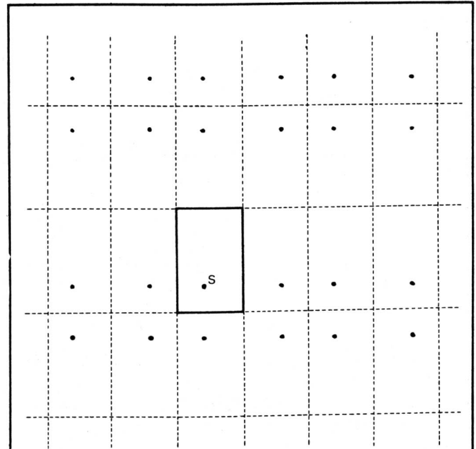
Figure 10. Phantom source patterns for a rectangular room form perfectly regular patterns of rows and columns. Any room shape which tessellates a surface by reflecting across each of its edges will have such a repeating pattern of sources. Such figures include equilateral triangles, for instance, and regular hexagons.
