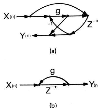
Figure 1. The simplest unit reverberators: (a) one-multiply all-pass; (b) comb filter. The magnitude of g must be less than 1 for stability.
